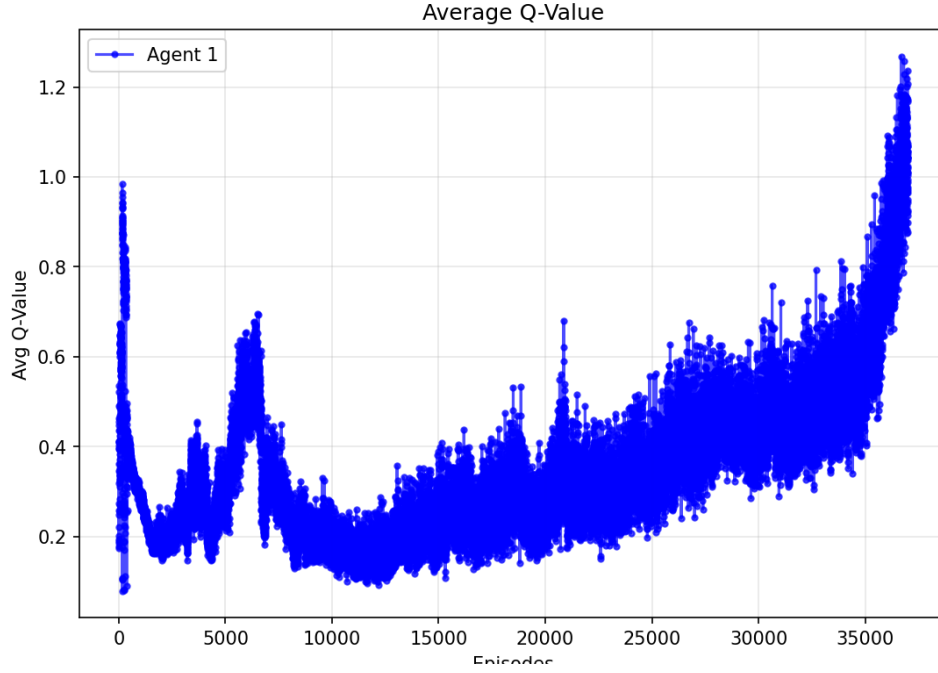
Figure 5.3: Average Q-values climb.
