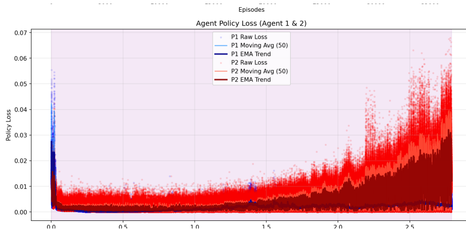
Figure 5.2: Policy loss (TD error).
