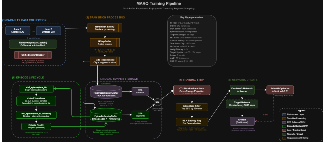
Figure 4.2: MARQ training architecture.
