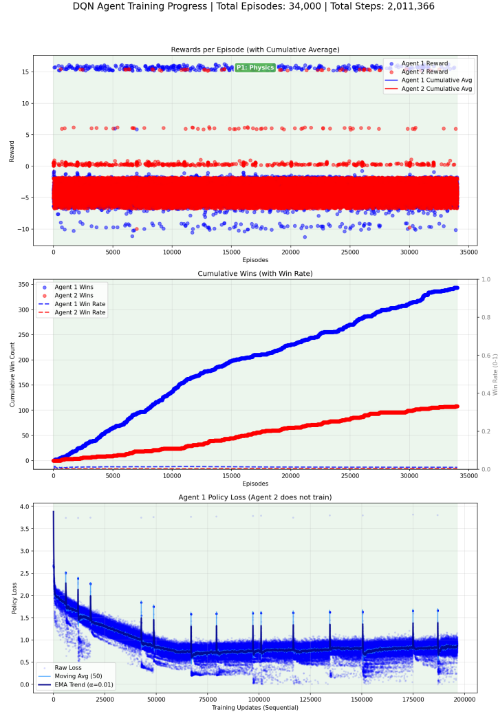
Figure B.8: Training Progress: Episode 34,000
