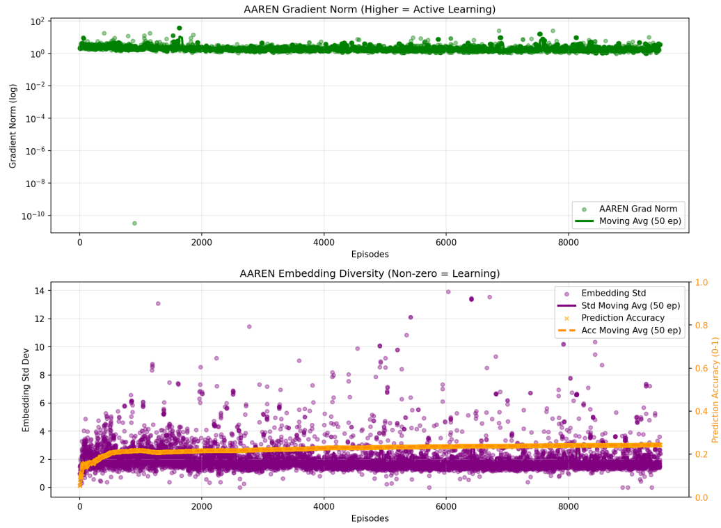
Figure B.14: AAREN End-to-End Training Metrics at 9,778 Episodes
