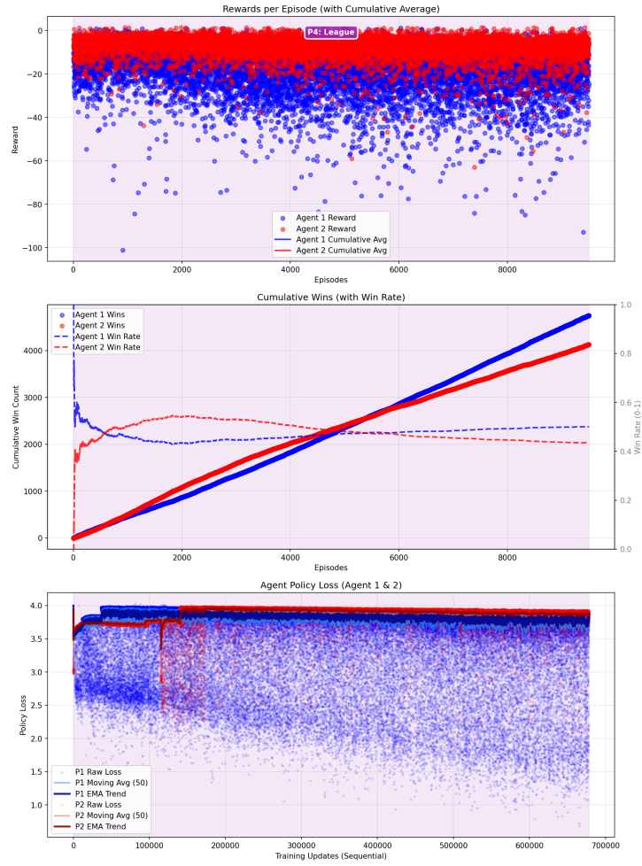
Figure B.12: Rainbow DQN+AAREN Training Progress at 9,778 Episodes
