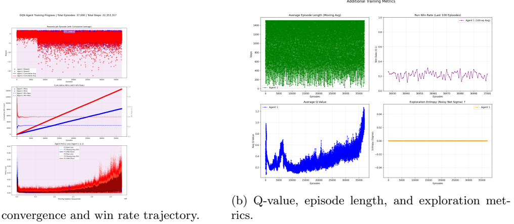
Figure 5.2: Training diagnostics at episode 37,000. The win rate (dashed blue line) remains at approximately 22% despite continued training, while Q-values exhibit an upward trend decoupled from performance. The Noisy Net sigma remains at zero throughout, indicating no learned exploration.
