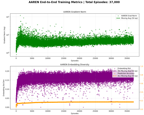
Figure 5.3: AAREN/LSTM training metrics at episode 37,000. The prediction accuracy (orange line) plateaus at approximately 18–22% after episode 5,000, while gradient norms remain stable, suggesting the module has converged to a local optimum.
