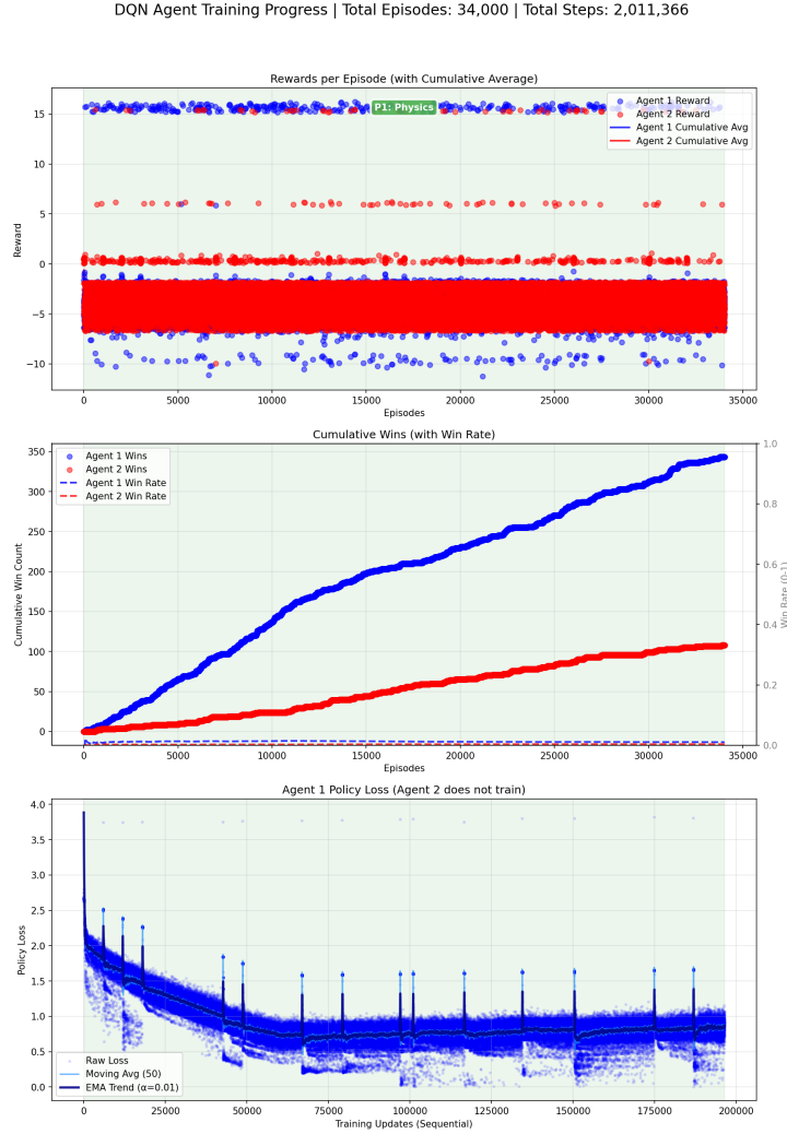
Figure B.10: Training Progress: Episode 34,000
