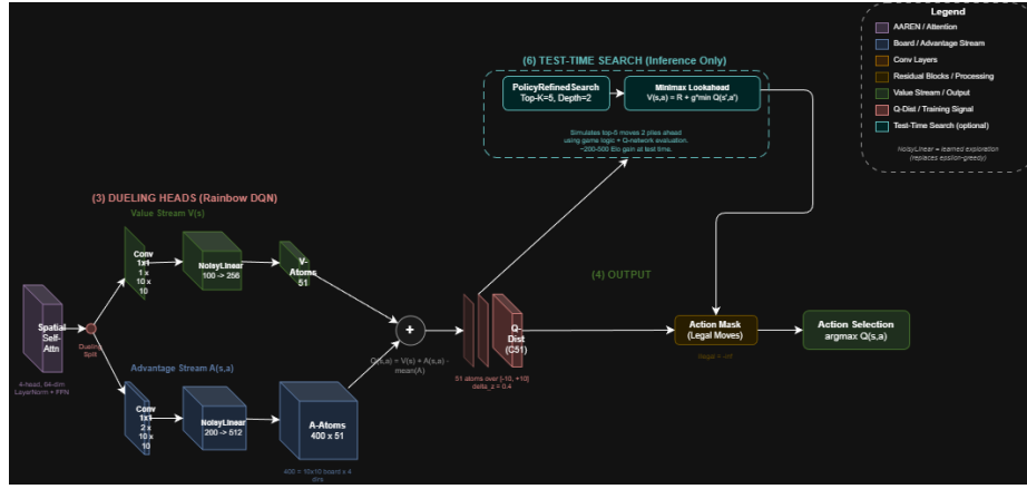
Figure 4.3: Dueling Network Heads. The architecture separates the value stream V(s) and the advantage stream A(s, a) , allowing the agent to stabilize learning by identifying state importance independently of action selection.
