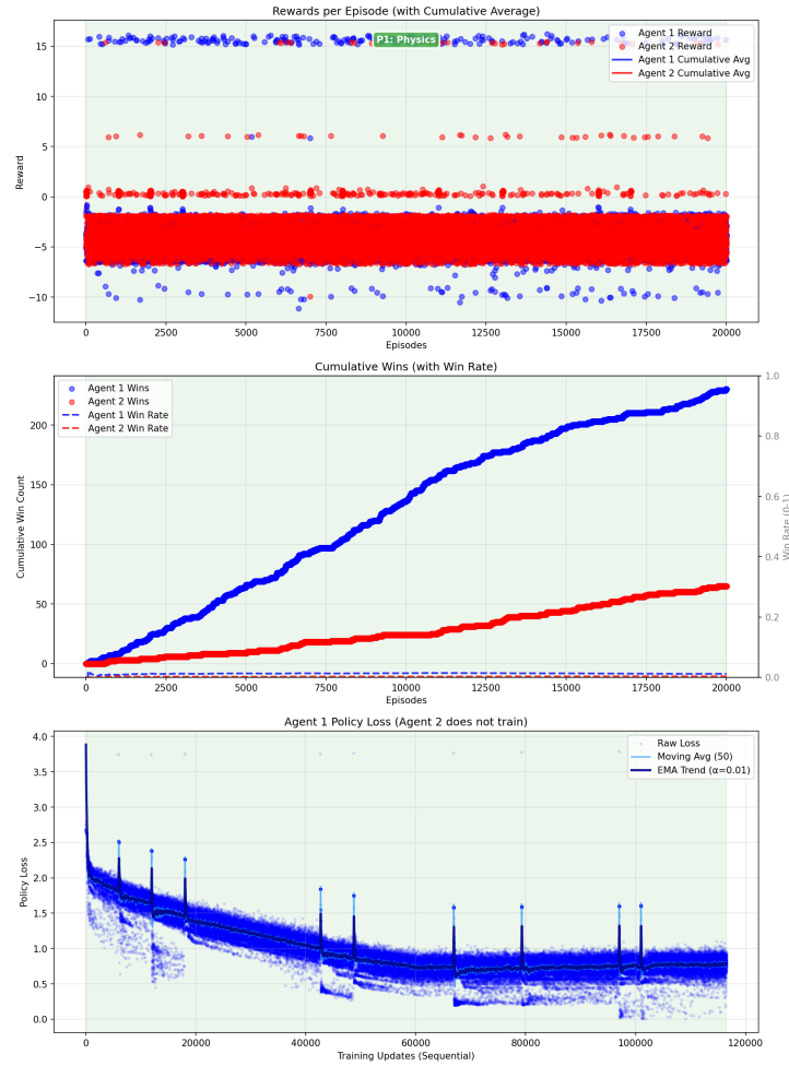
Figure B.9: Training Progress: Episode 20,000
