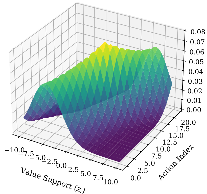
C51 Distributions Across Actions
