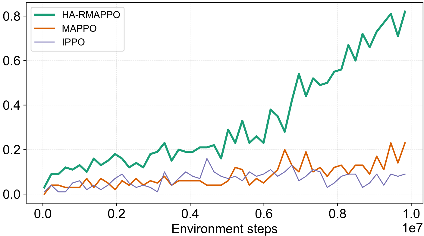
Defense success rate
