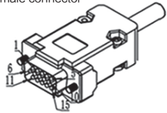
DB three-row 15-pin male connector
