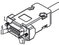
DB three-row 15-pin male connector
