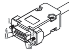
DB three-row 15-pin male connector
