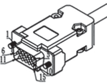
DB three-row 15-pin male connector
