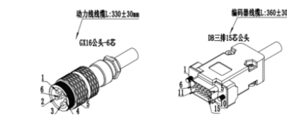
Wiring Definition of Incremental 2500-line Magnetic Encoder
