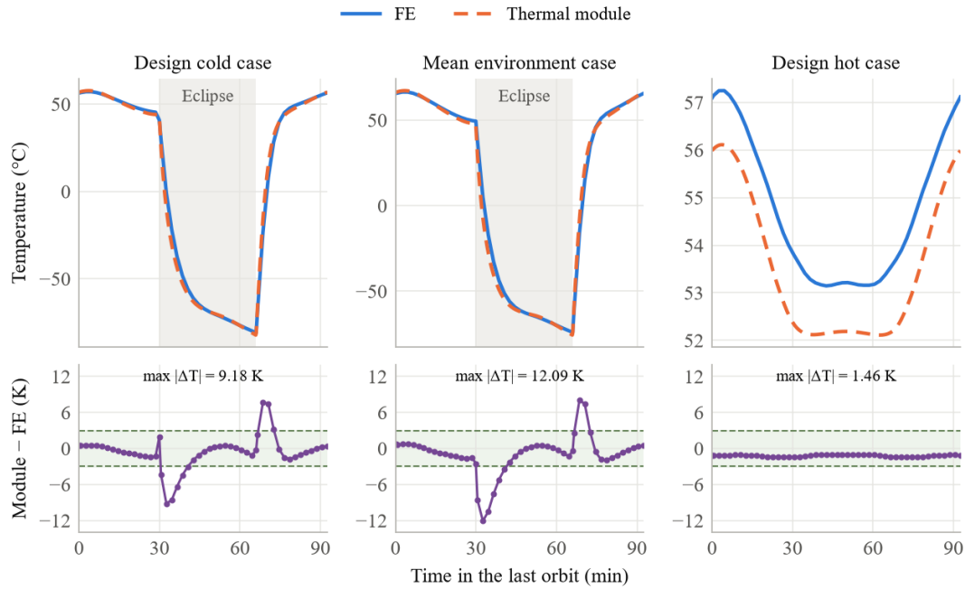
Figure 1. FE-001 solar array temperatures over the last orbit
