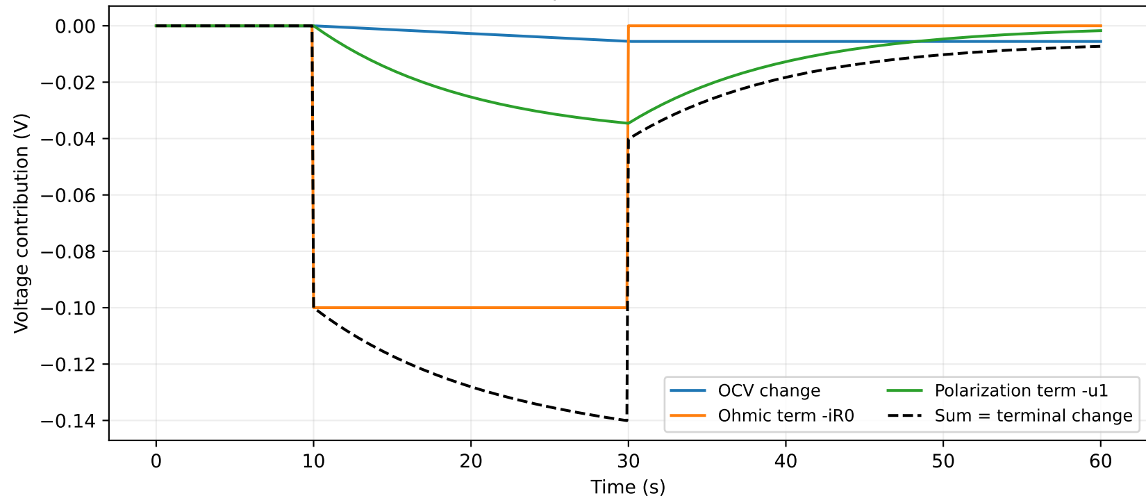
BT02 | V = \text{OCV} - iR_0 - u_1
