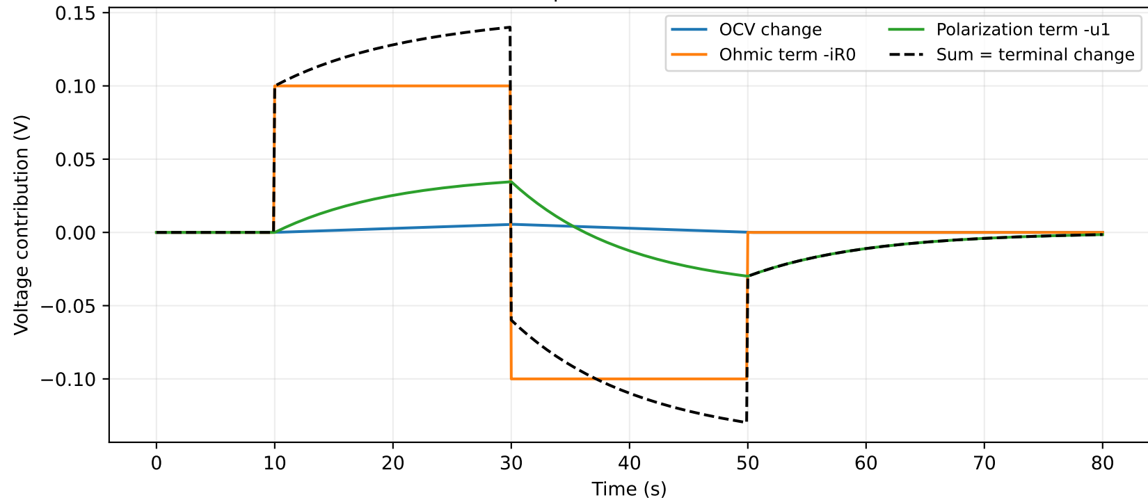
BT03 | V = \text{OCV} - iR_0 - u_1
