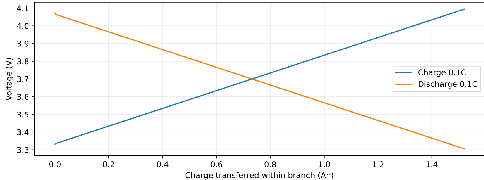
BT06 | SOC 0.12 to 0.88 and back; no accelerated physical time
