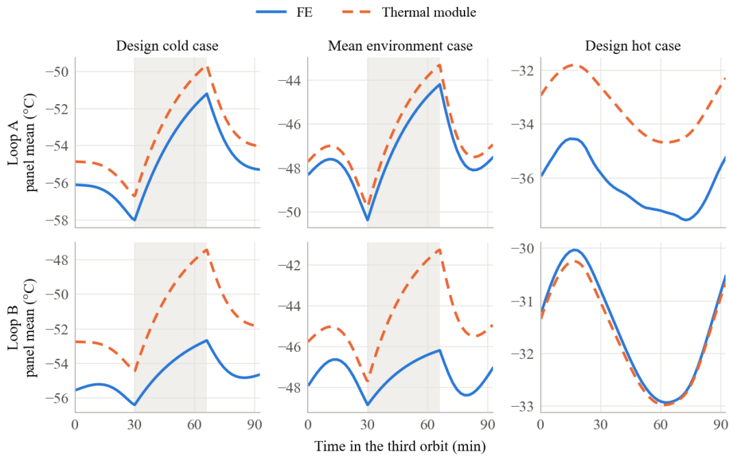
Figure 2. FE-002 common radiator temperatures over the third orbit
