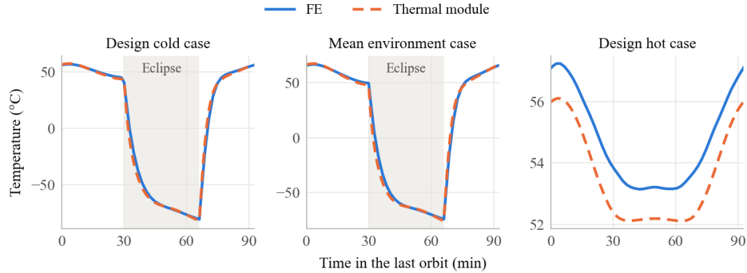
Figure 1. FE-001 solar array temperatures over the last orbit
