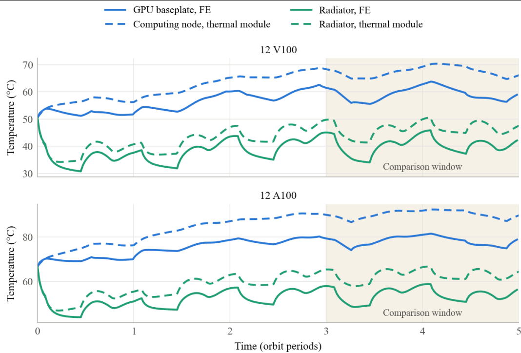
Figure 3. FE-004 GPU baseplate, computing node and radiator temperature histories
