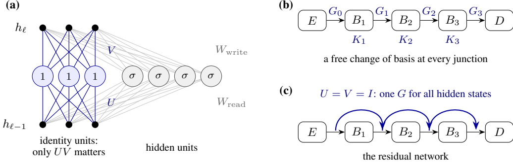
Figure 1: (a) A mixed vanilla MLP block with d_{\text{model}} = 3 identity units and 4 hidden units, drawn as one wide layer: its read places U and W_{\text{read}} side by side, its map is [\text{Id}, \text{Id}, \text{Id}, \sigma, \sigma, \sigma, \sigma] , and its write stacks V and W_{\text{write}} . Nothing nonlinear happens between the read U and the write V of the identity units, so only UV enters the function (Proposition 1). (b) A network of such blocks, or of blocks without identity units, between an embedding E and a readout D : each hidden state has a free change of basis G_{\ell} , and the identity units of each block a free K_{\ell} . (c) Spending them sets U = V = I in every block, which is the residual network (Theorem 2); the frozen identity units carry each hidden state into the next in the same basis, so one change of basis is left for all hidden states.
