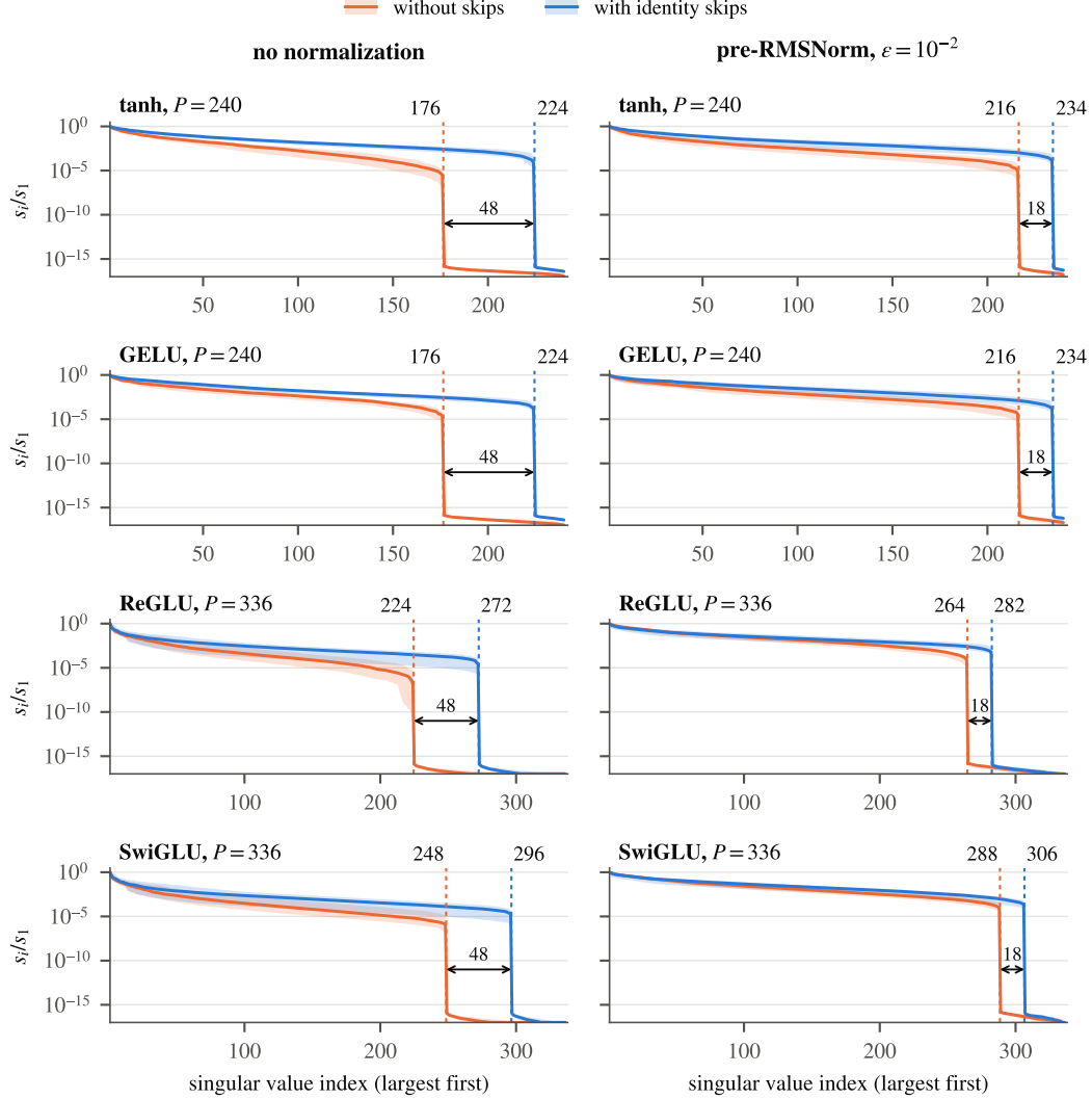
Figure 2: Singular values of the exact Jacobian of the parameter-to-output map, on 4000 inputs, for the same weights with and without identity skips: an embedding \mathbb{R}^6 \rightarrow \mathbb{R}^4 , L = 3 MLP blocks of width 8 and a readout \mathbb{R}^4 \rightarrow \mathbb{R}^6 , without biases. Left column: without normalization. Right column: with pre-RMSNorm, \varepsilon = 10^{-2} , before every block and the readout. Lines show the median over 20 random draws, and bands the range. The rank on the batch is a lower bound on the functional dimension, and the symmetry count P - (L + 1) \dim \mathcal{G} - s without skips and P - \dim \mathcal{G} - s with them an upper bound, with \dim \mathcal{G} = d_{\text{model}}^2 = 16 without normalization and d_{\text{model}}(d_{\text{model}} - 1)/2 = 6 under RMSNorm; the dashed lines mark the two counts, and the arrows their difference. In every draw the rank, read at a gap of at least 10^4 , equals the count, so the skips add L \dim \mathcal{G} : 48 without normalization and 18 under RMSNorm.
