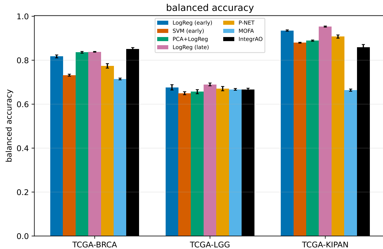
Overall full-data performance across datasets
