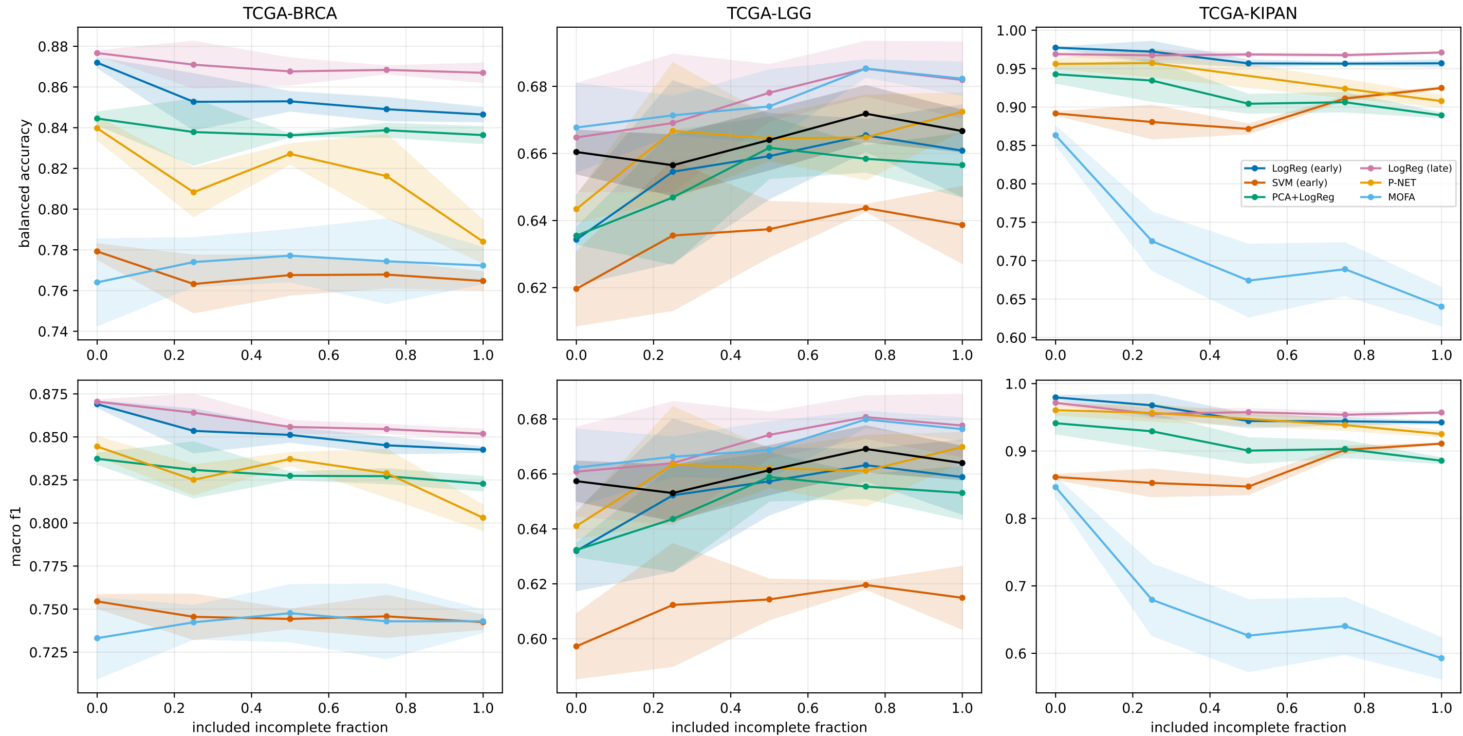
Primary metrics vs random omic missingness
