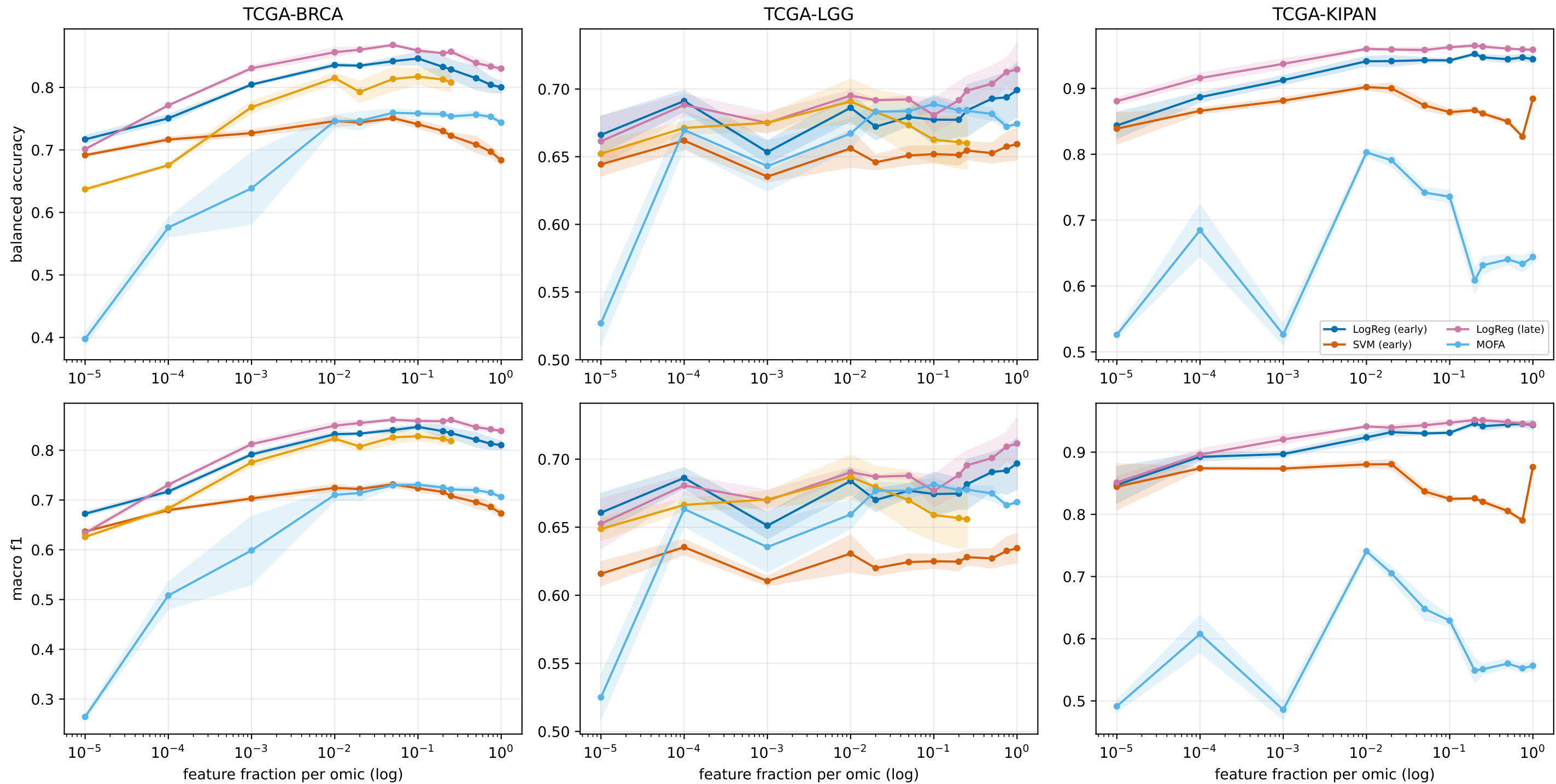
Primary metrics vs percentage of features
