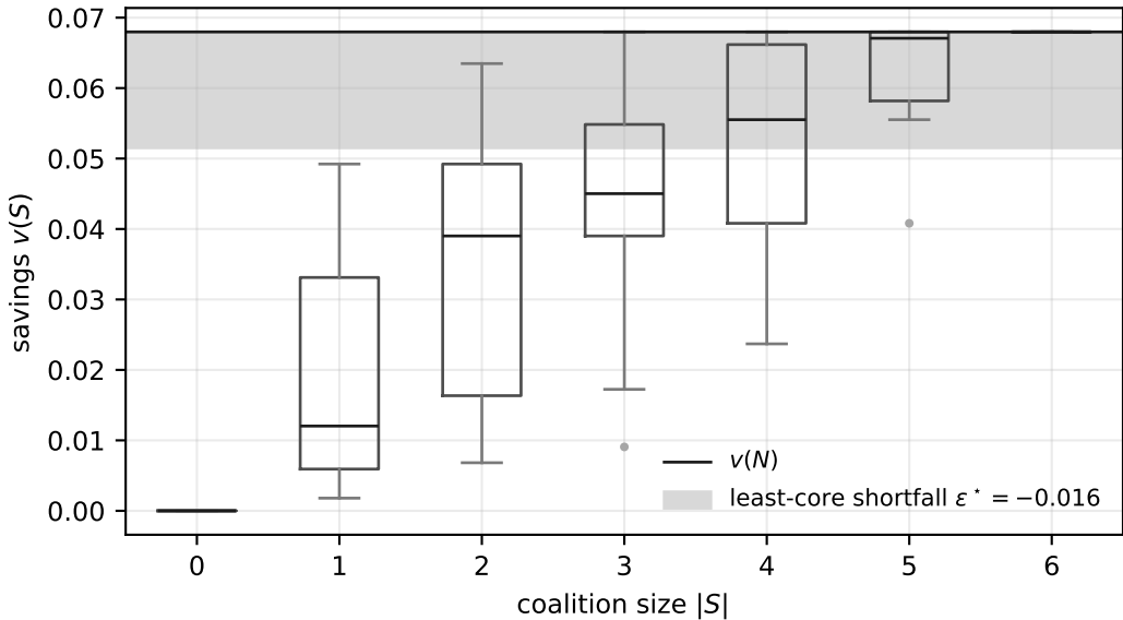
EX11: savings by coalition size
