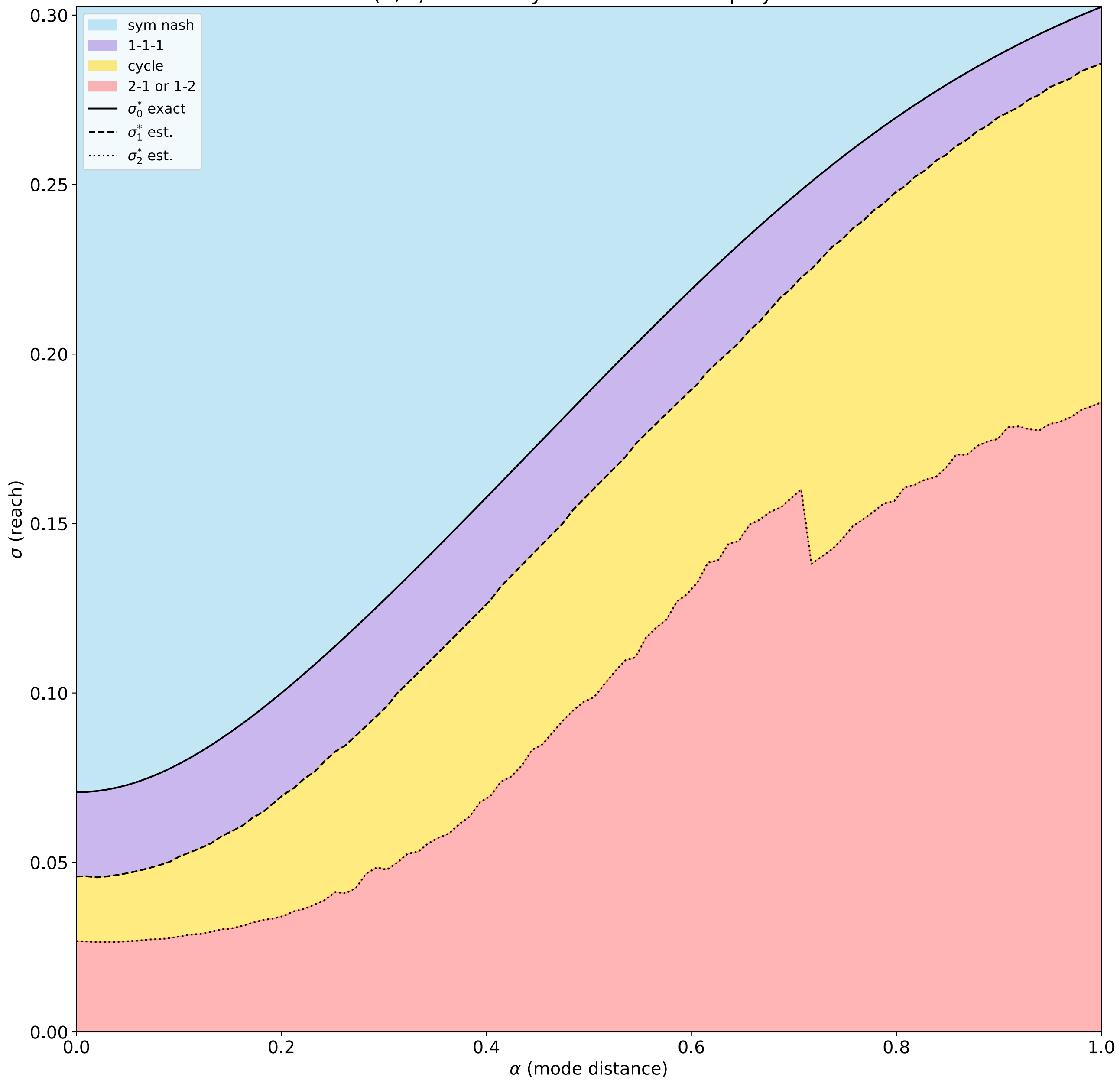
(\alpha, \sigma) x^* stability bifurcation for 3 players
