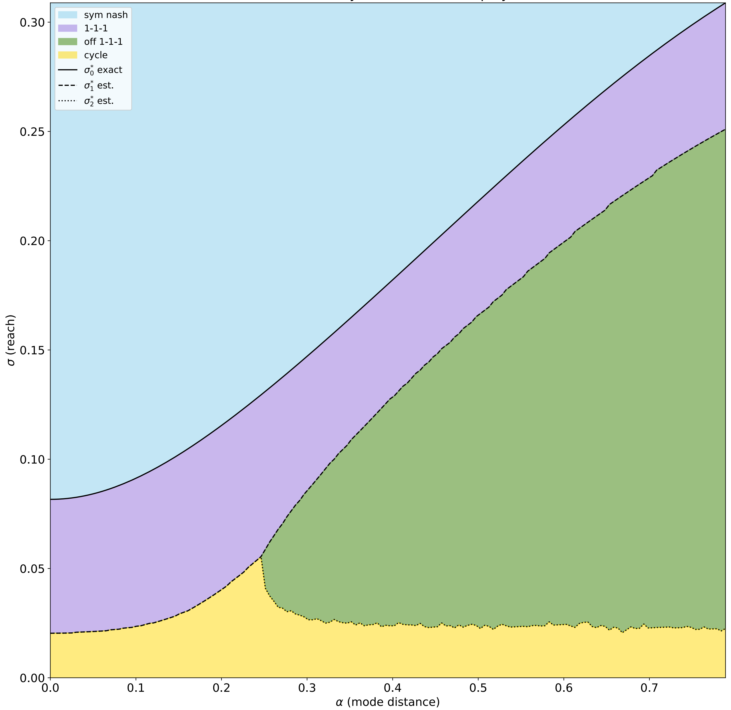
(\alpha, \sigma) x^* stability bifurcation for 4 players
