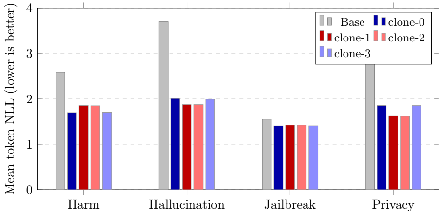
Fixed-theory specialists vs base (round 39, 10 seeds)
