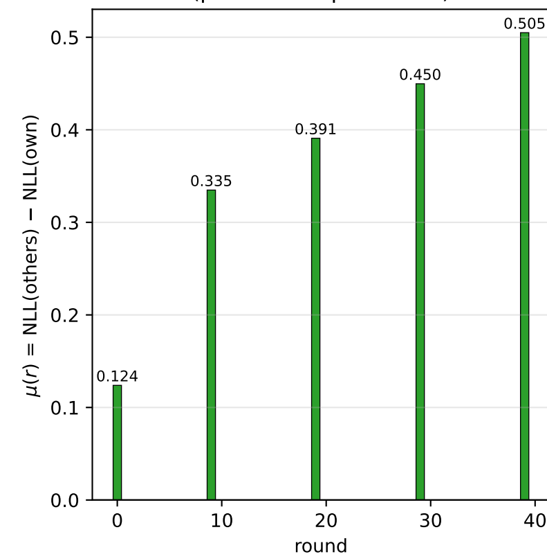
Tier 3c — specialisation margin (positive = specialised)
