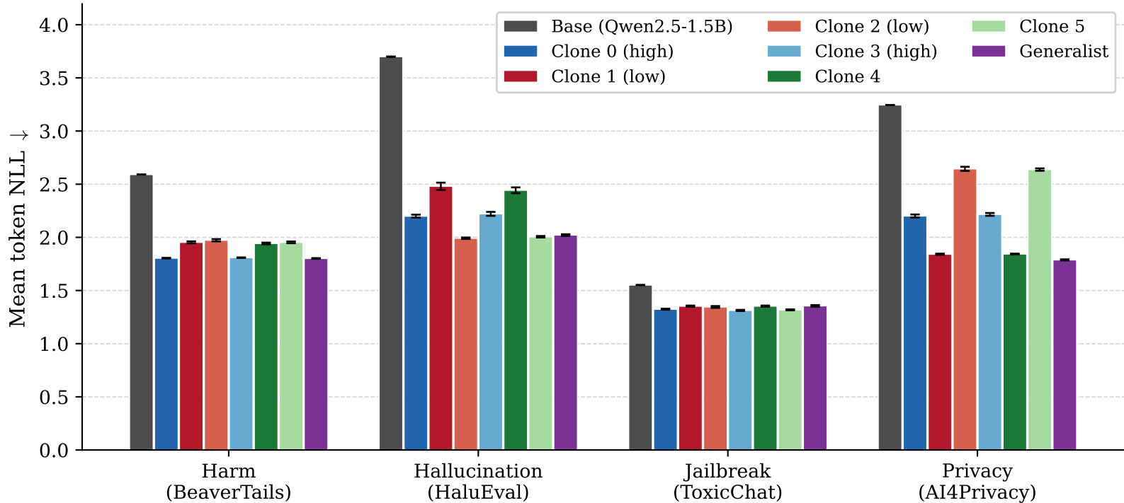
Fixed-theory specialists vs base vs generalist (round 9, sigma=0.25, 10 SFT seeds, 10 specialist seeds, 10 generalist seeds)
