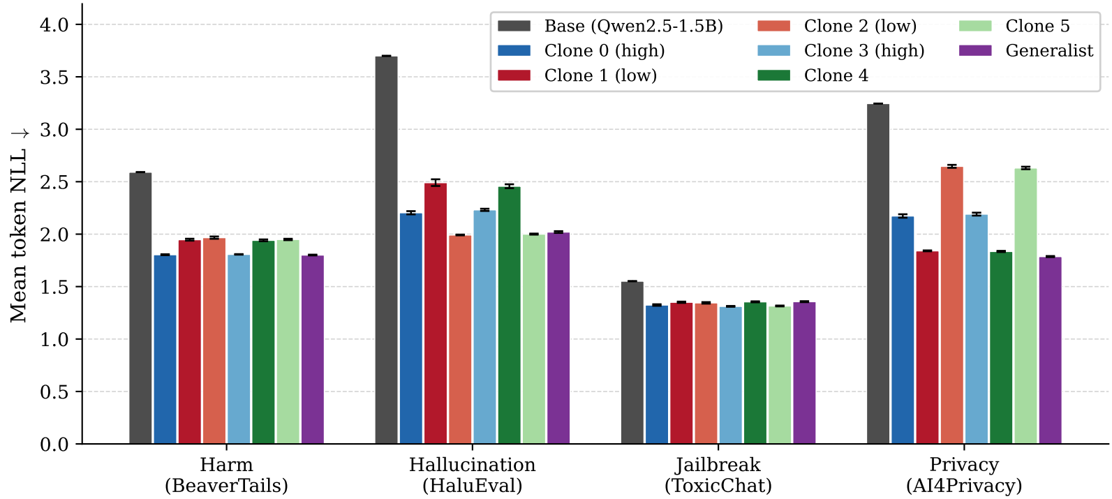
Fixed-theory specialists vs base vs generalist (round 9, sigma=0.5, 10 SFT seeds, 10 specialist seeds, 10 generalist seeds)
