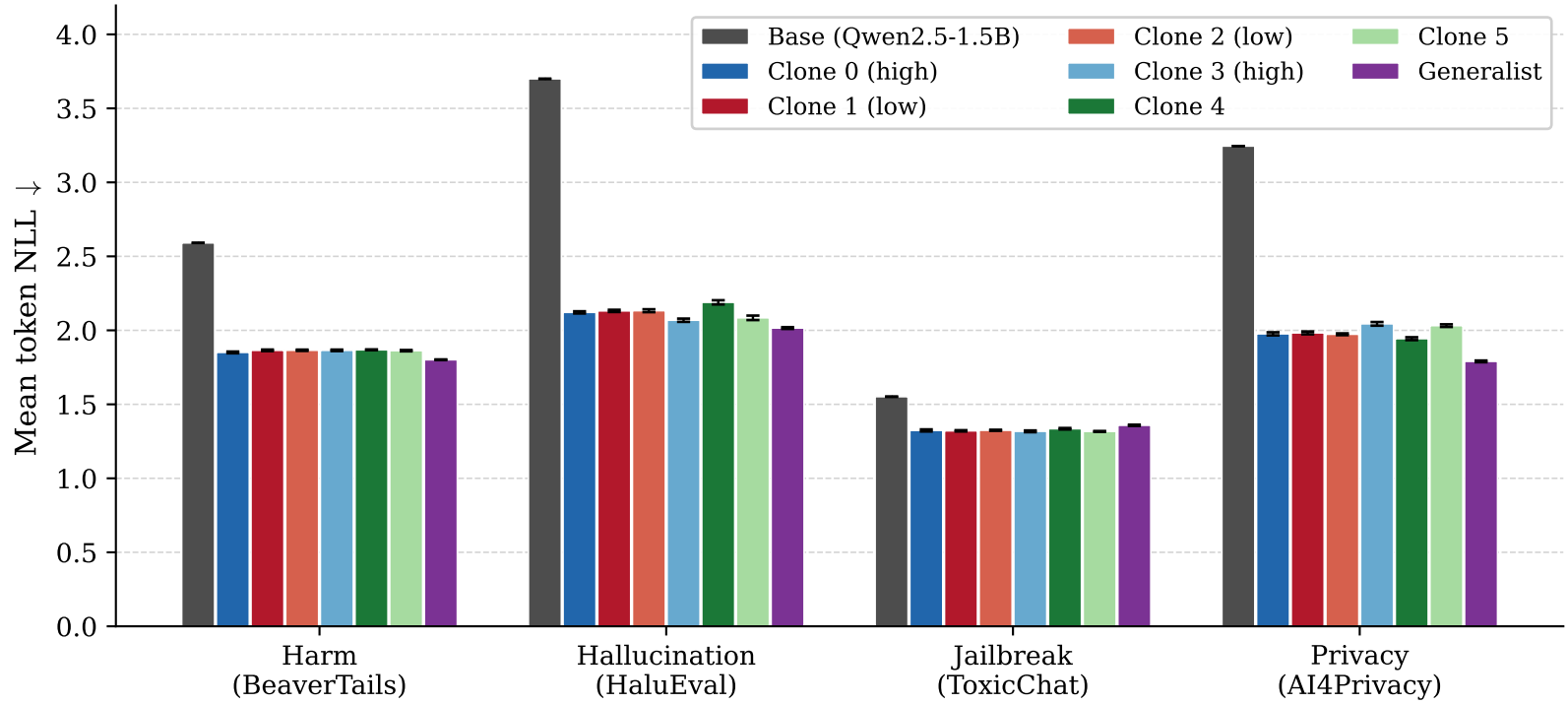
Fixed-theory specialists vs base vs generalist (round 9, sigma=1.0, 10 SFT seeds, 10 specialist seeds, 10 generalist seeds)
