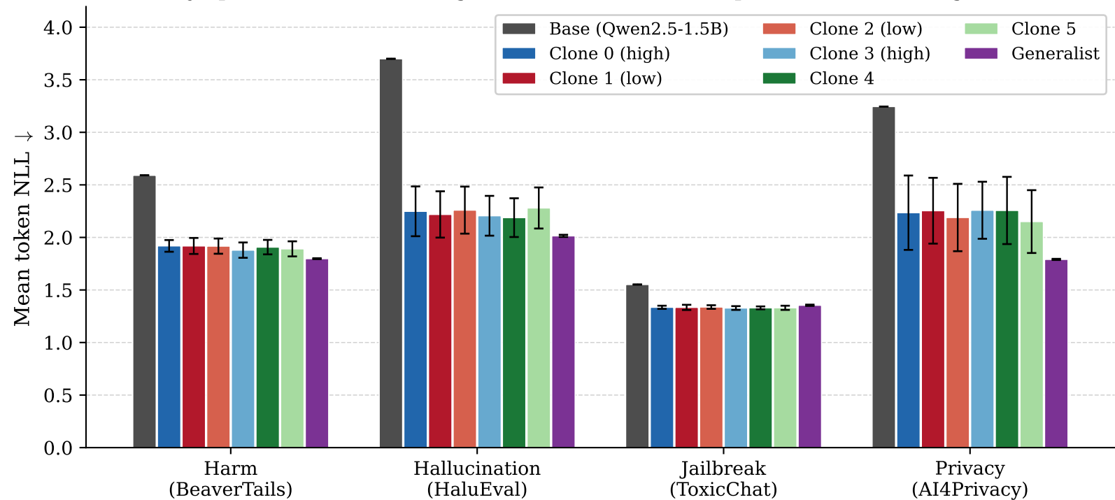
Fixed-theory specialists vs base vs generalist (round 9, 10 specialist seeds, 10 generalist seeds)
