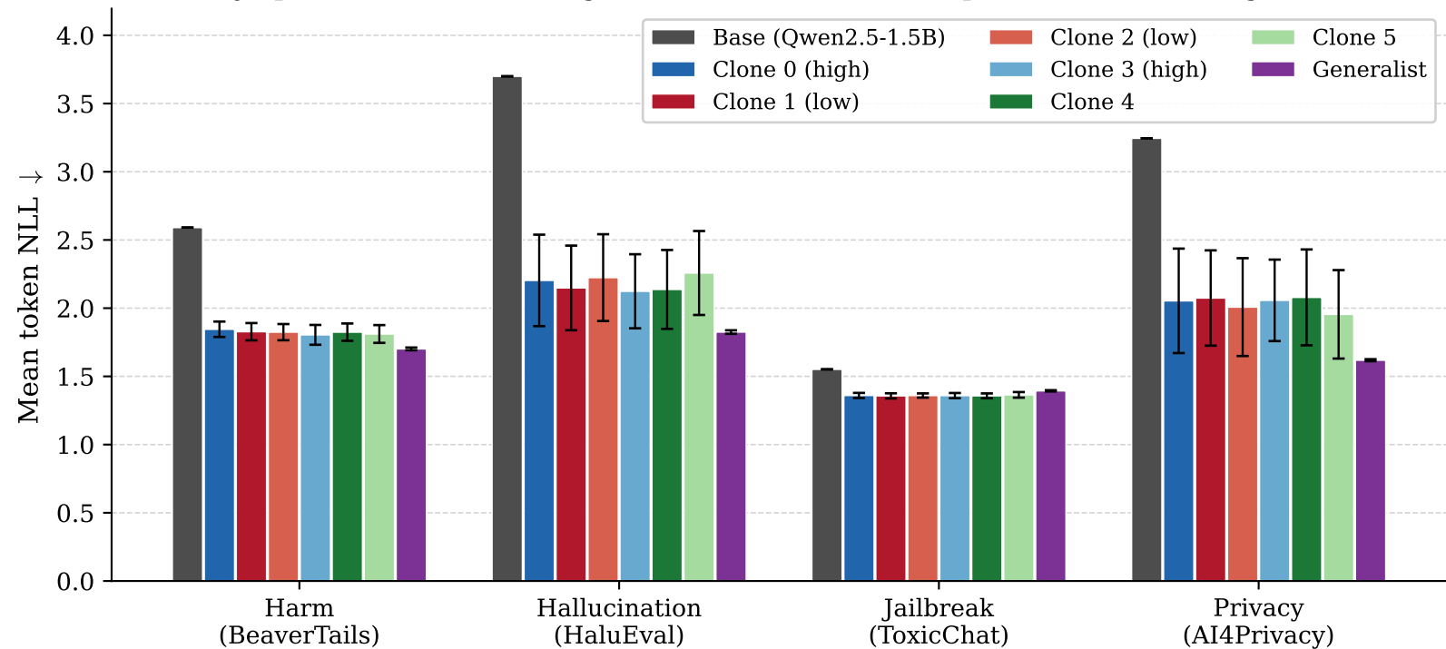
Fixed-theory specialists vs base vs generalist (round 39, 10 specialist seeds, 10 generalist seeds)
