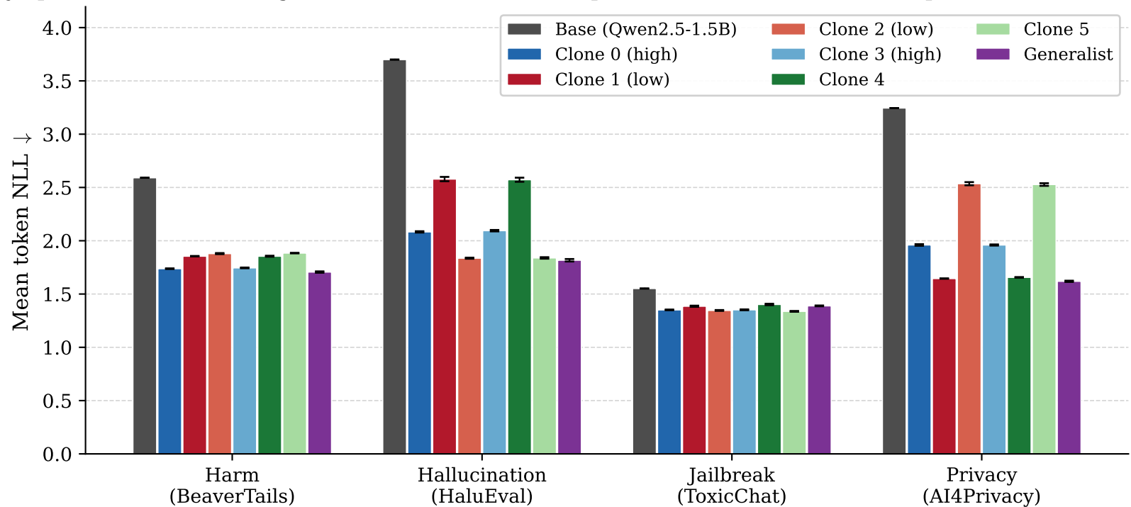
Fixed-theory specialists vs base vs generalist (round 39, fixed positions, 10 SFT seeds, 10 specialist seeds, 10 generalist seeds)
