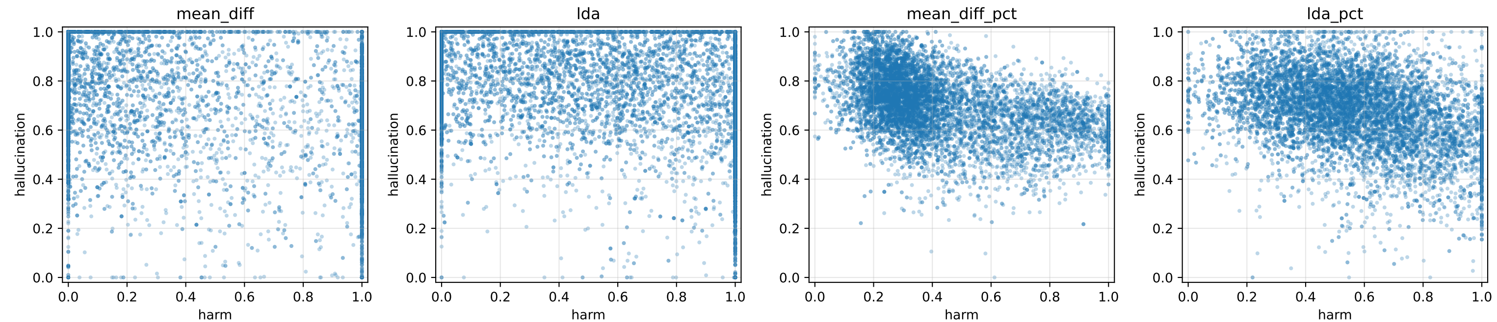
Calibrated trait coordinates by axis estimator
