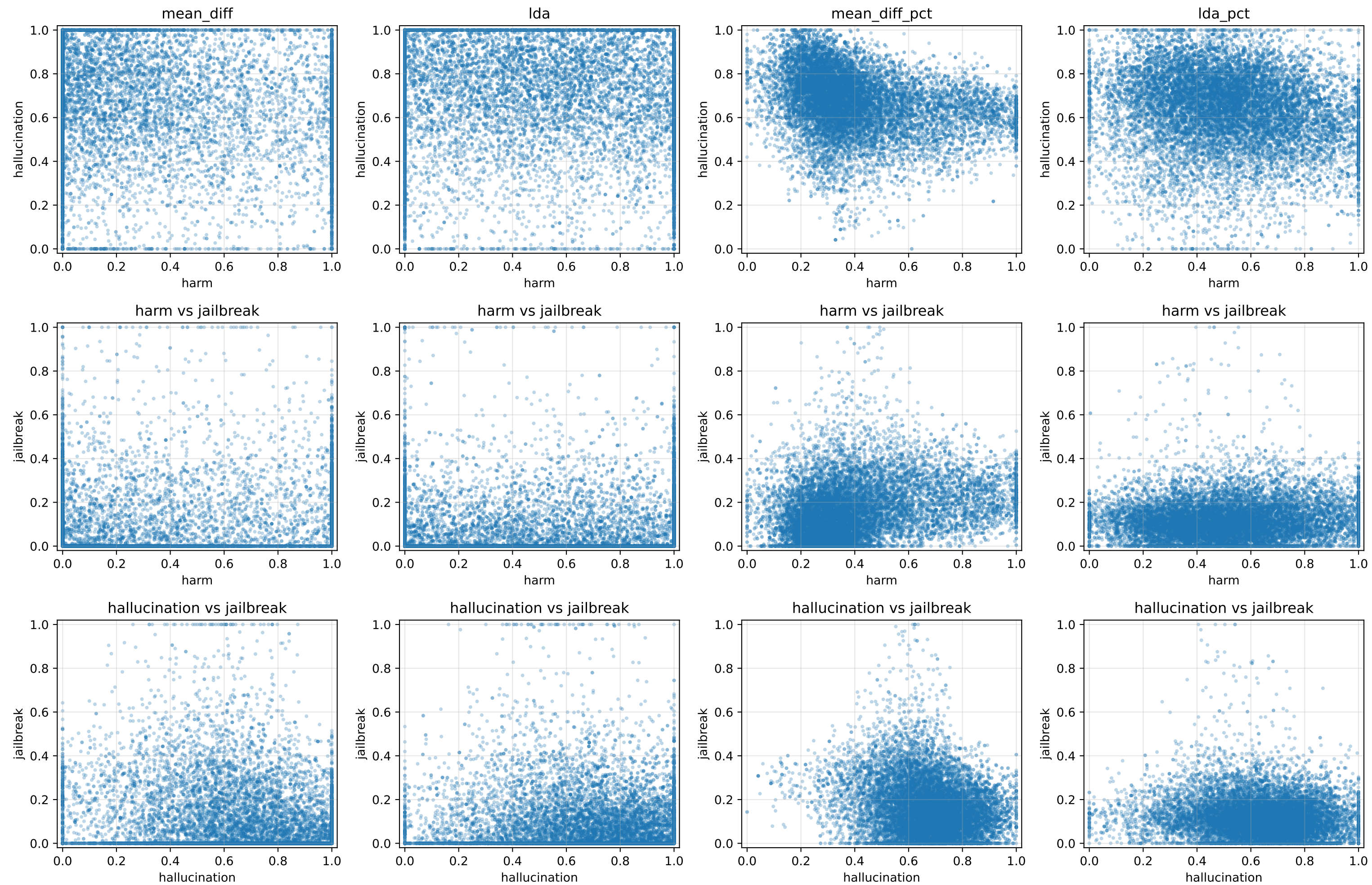
Calibrated trait coordinates by axis estimator
