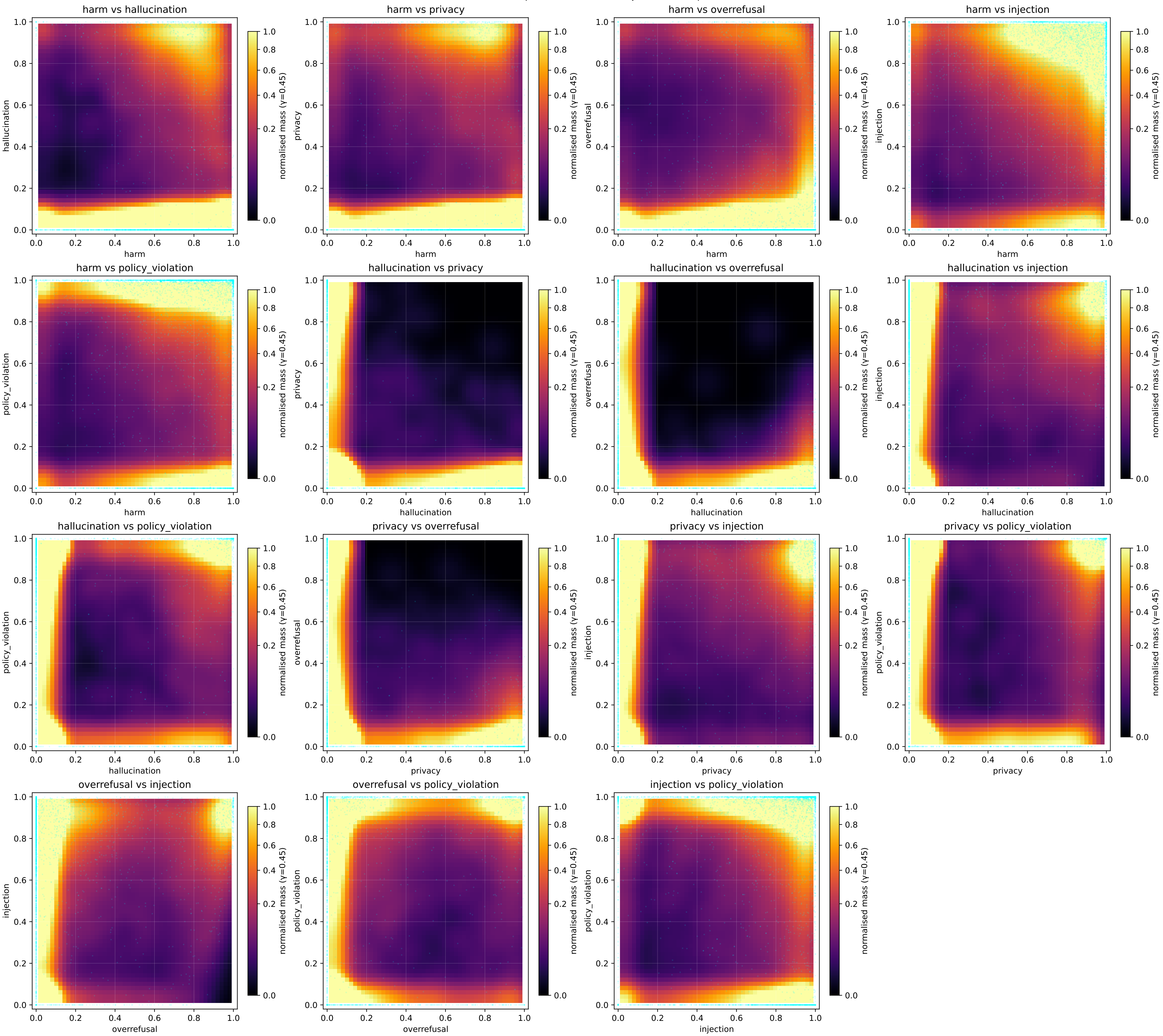
Six-axis trait space (Threat Matrix injection, 5k cap)
