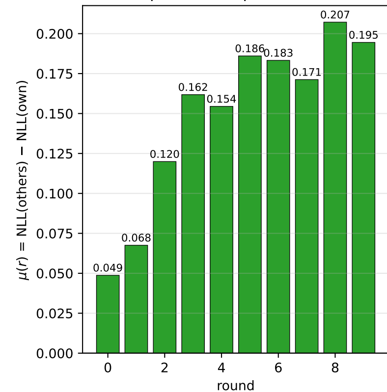
Tier 3c — specialisation margin (positive = specialised)
