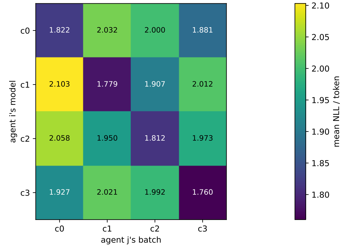
Tier 3a — cross-NLL at round 9
