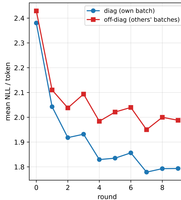
Tier 3b — fit on own vs others' batches
