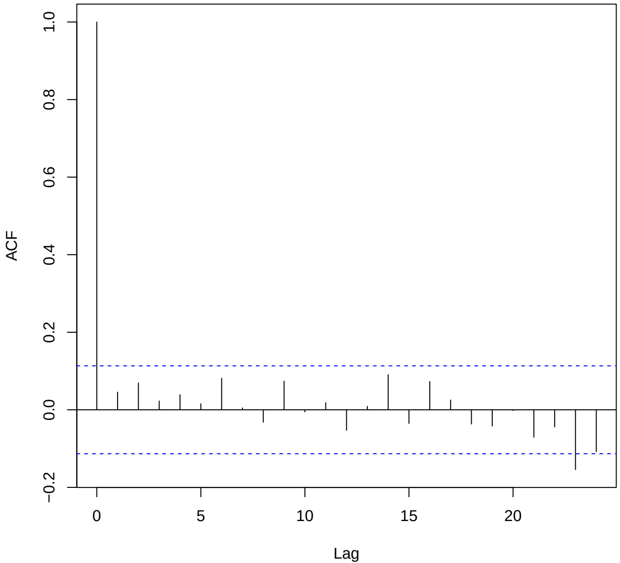
Series diff(signal)
