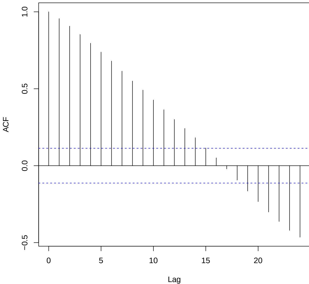
Series signal
