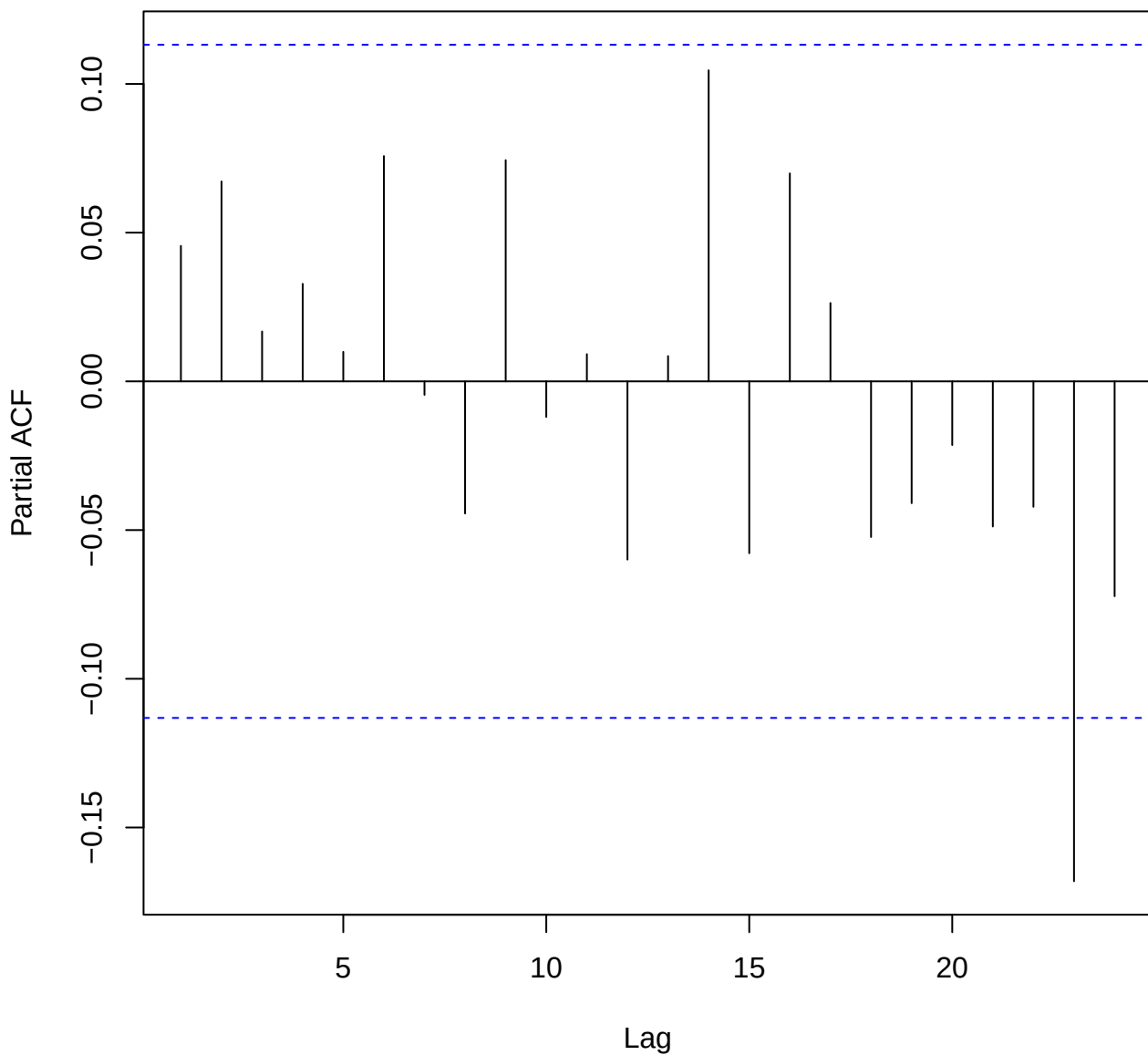
Series residuals(a1)
