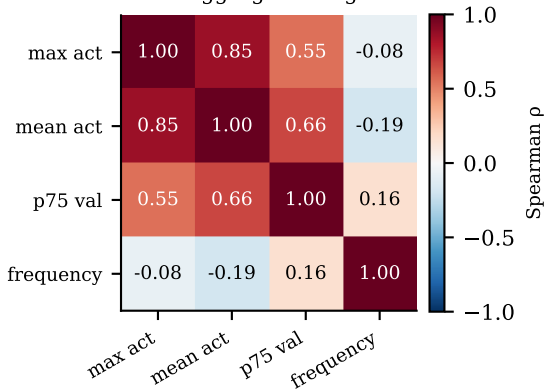
Rank correlation between MEI aggregation signals
