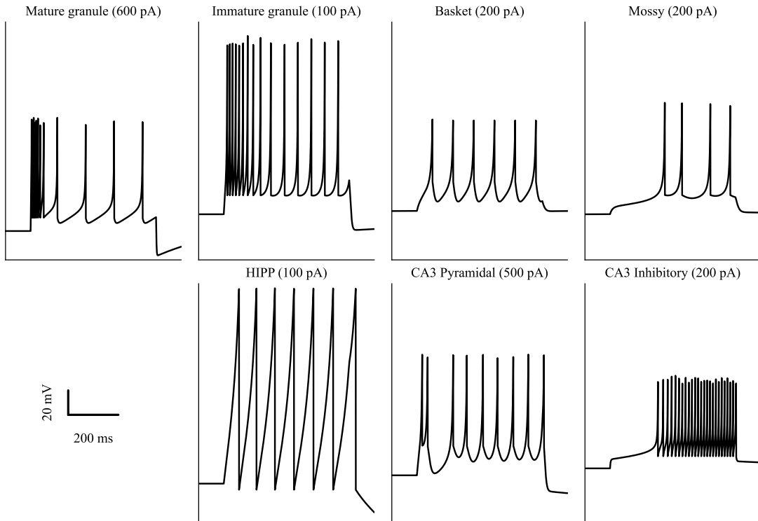
Figure 3 – Spike traces of neurons under constant current as indicated by each subfigure title.
