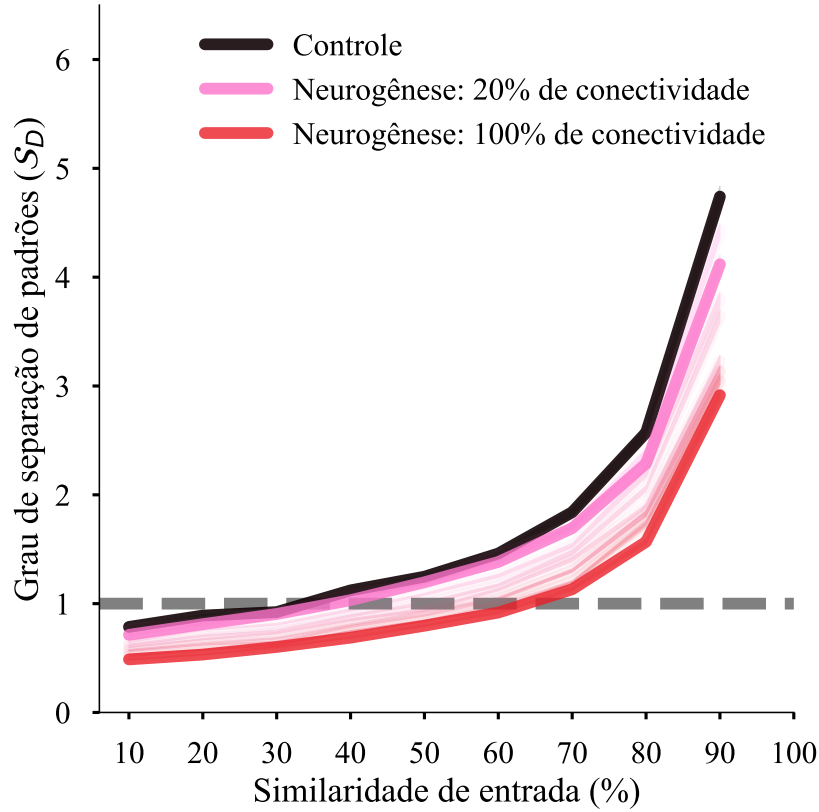
Figure 6 – Degree of pattern separation ( \mathcal{S}_D ) per model and input similarity level. The dashed line represents a separation degree of 1; values above this indicate that pattern separation occurred, while values below indicate that it did not. Error is represented by the shaded area.
