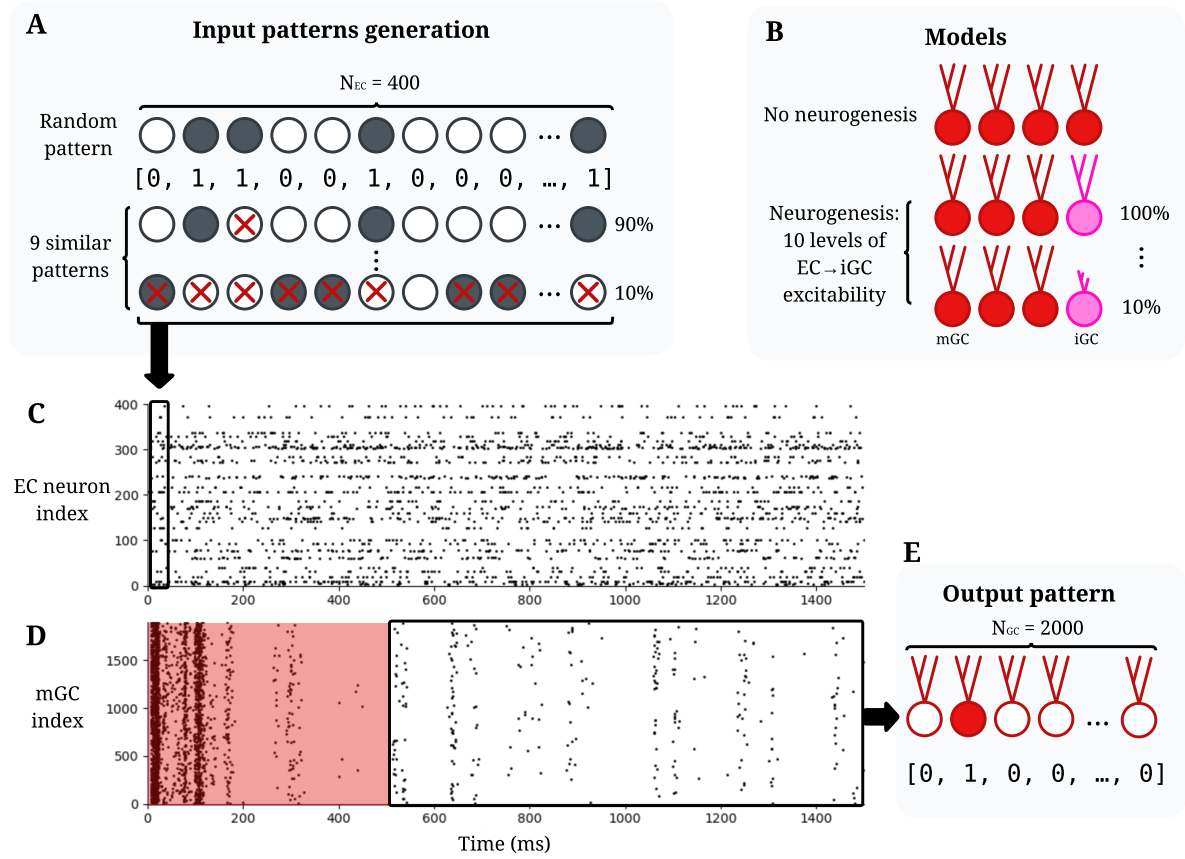
Figure 4 – Diagram of the input and output pattern generation and recall protocol. A. Input patterns are generated in sets of 10 patterns of size N_{EC} = 400 ; the first is generated randomly and the remaining ones are generated from it at different levels of similarity by randomly activating and deactivating neurons. B. 11 model variants are simulated: one without neurogenesis and 10 with neurogenesis at different connectivity levels, from 100% down to 10% connectivity. C. Spike trace of EC neurons during a simulation; each generated pattern corresponds to the activation of EC neurons, with active neurons spiking at a frequency of 40 Hz; each of the 11 models is exposed to 20 sets of 10 input patterns, totaling 200 simulations of 1500 ms each. D. Spike trace of mGCs during a simulation; the first 500 ms are discarded while the network stabilizes; the remainder corresponds to the output pattern. E. The output pattern, illustrated here for the mGC population, consists of a binary vector with value 1 for the index of each neuron that spiked at least once during the 1000 ms interval.
