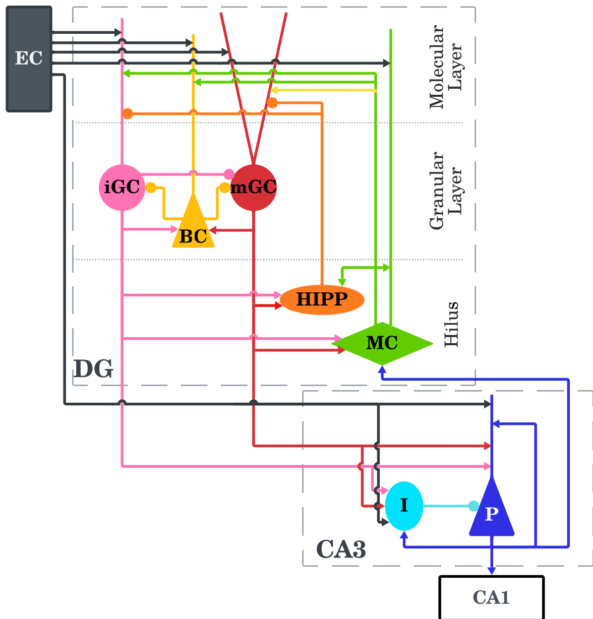
Figure 1 – DG-CA3 network architecture. Inhibitory synapses are represented by circles and excitatory ones by arrows. The network input is composed of cells from the entorhinal cortex (EC). The dentate gyrus (DG) has the perforant path and the dendrites of its cells in the molecular layer; the granular layer is composed of immature and mature Granule Cells (iGCs and mGCs, respectively) and Basket Cells (BCs); the hilus is composed of Mossy Cells (MCs) and Hilar Perforant Path-associated cells (HIPPs). The CA3 is composed of pyramidal CA3 cells (pCA3) and inhibitory CA3 cells (iCA3).
