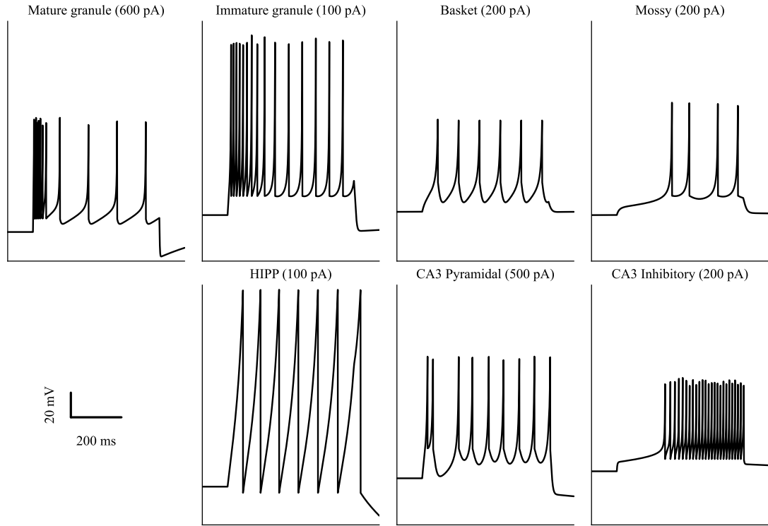
Figure 3 – Spike traces of neurons under constant current as indicated by each subfigure title.
