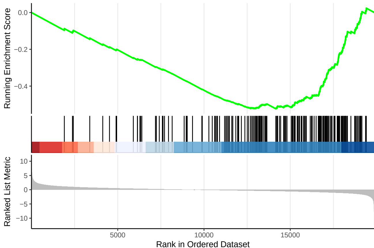
Chutake_0.05_all_genes.rds GO CC ribosomal subunit
