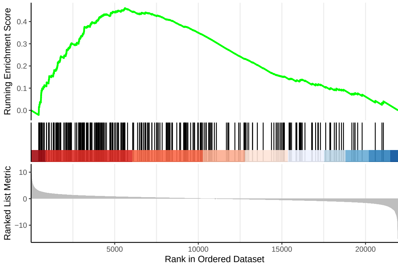
Wang_0.05_all_genes.rds GO CC condensed chromosome
