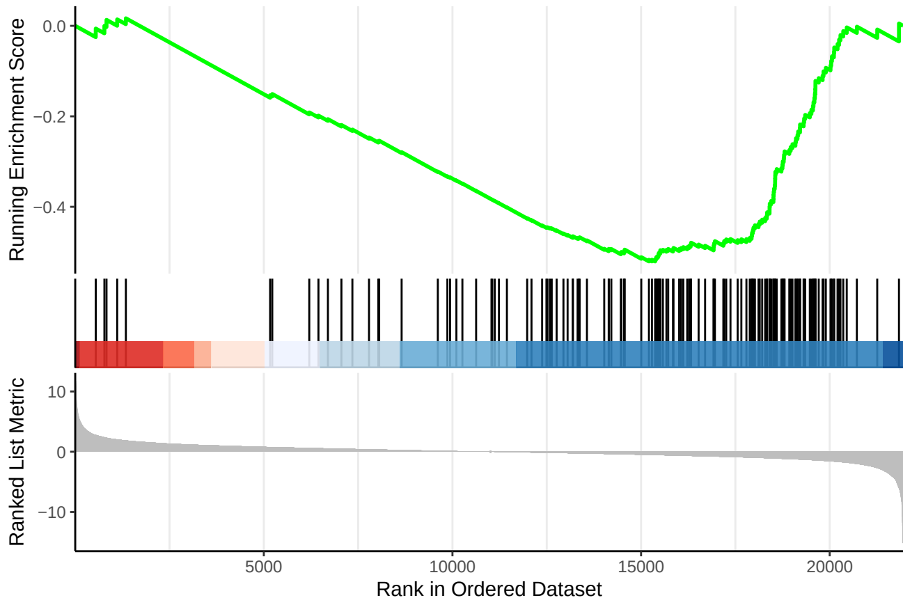
Wang_0.05_all_genes.rds GO MF structural constituent of ribosome
