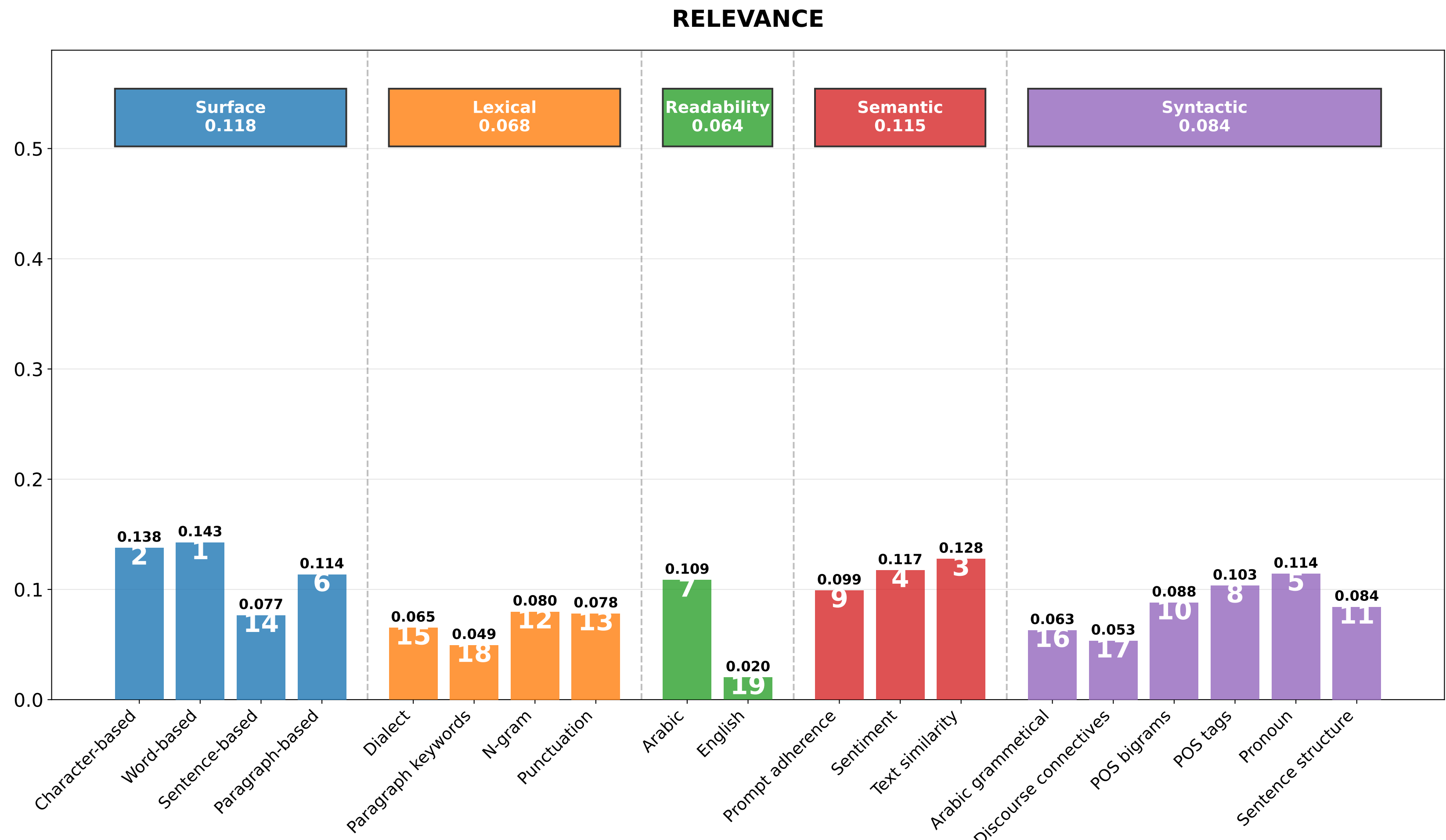
Complete Feature Set Correlations - Prompt 2
