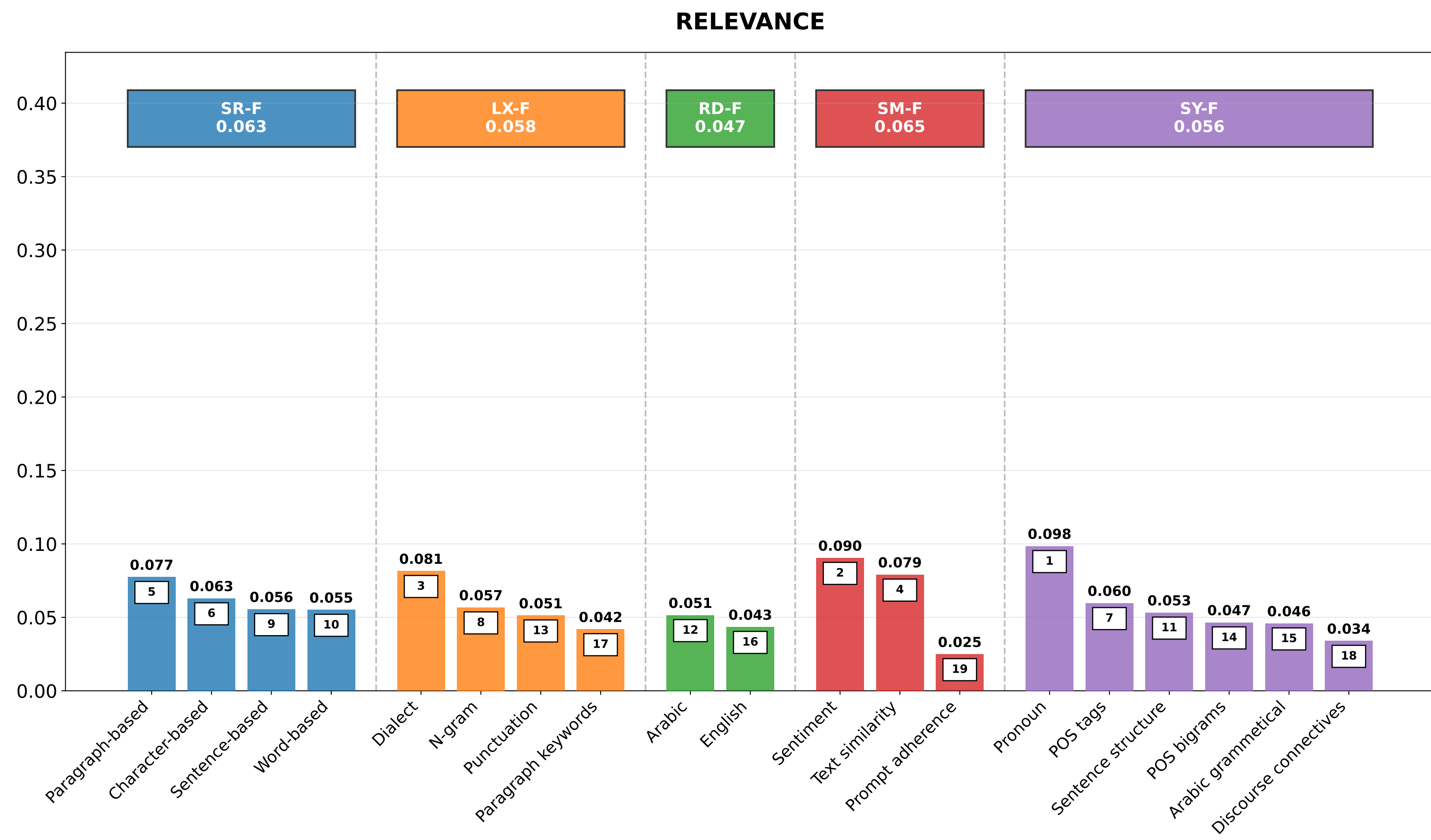
Complete Feature Set Correlations - Whole Dataset
