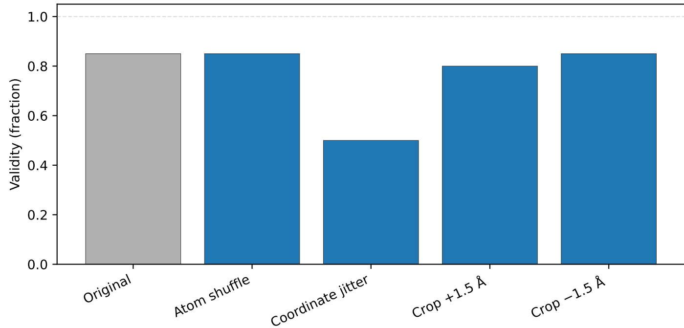
Pocket 3RFM: validity under invariant perturbations (DiffSBDD)
