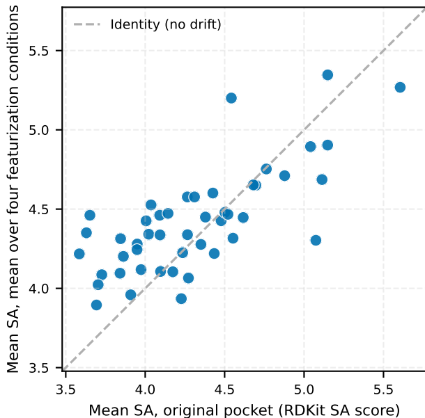
Mean synthetic accessibility drift (DiffSBDD, 47 pockets): 27/47 above identity
