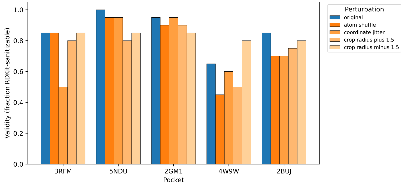
DiffSBDD validity by pocket and pocket-input perturbation
