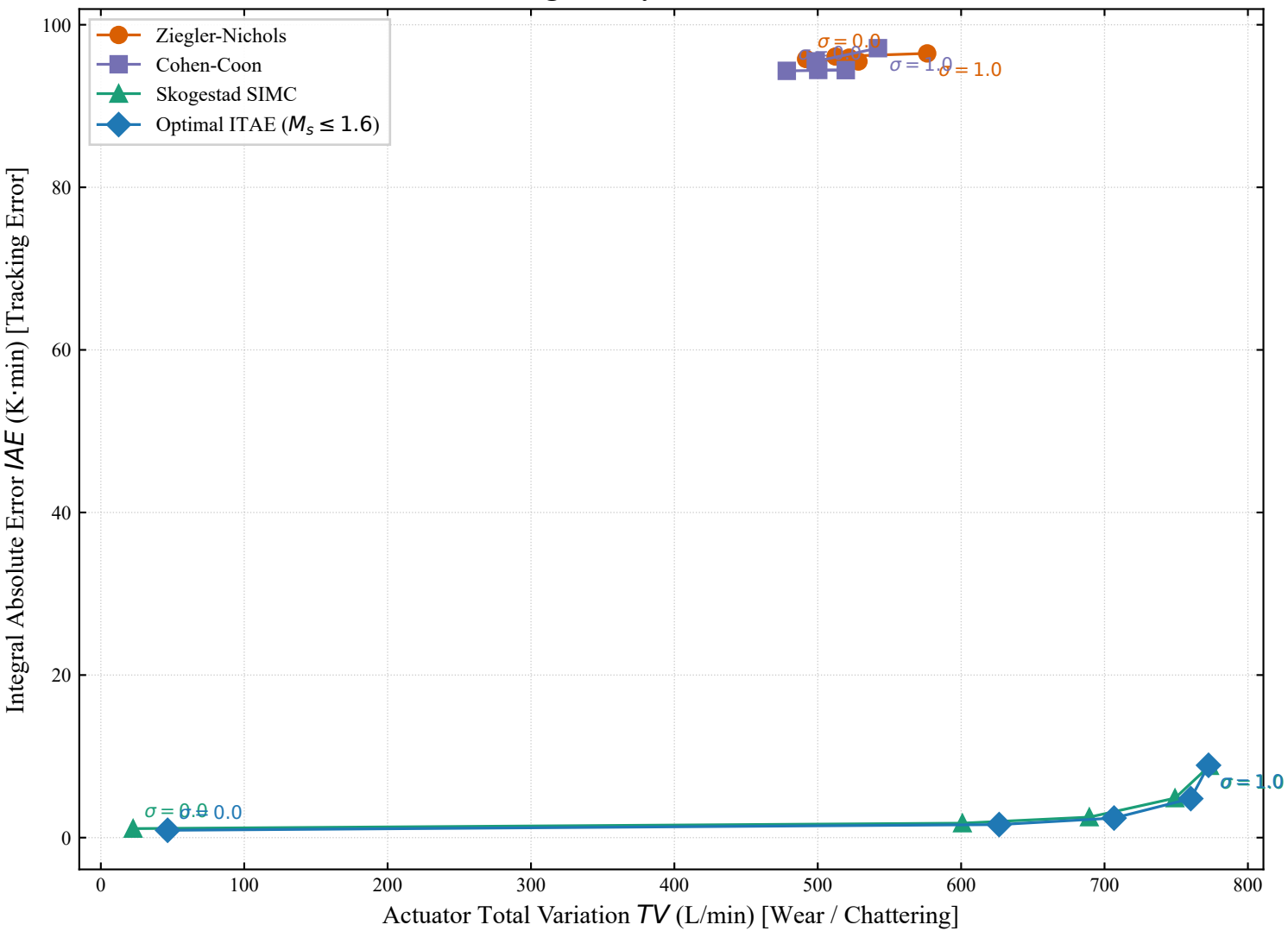
Pareto Trade-off: Tracking Quality vs Actuator Wear across Noise Levels
