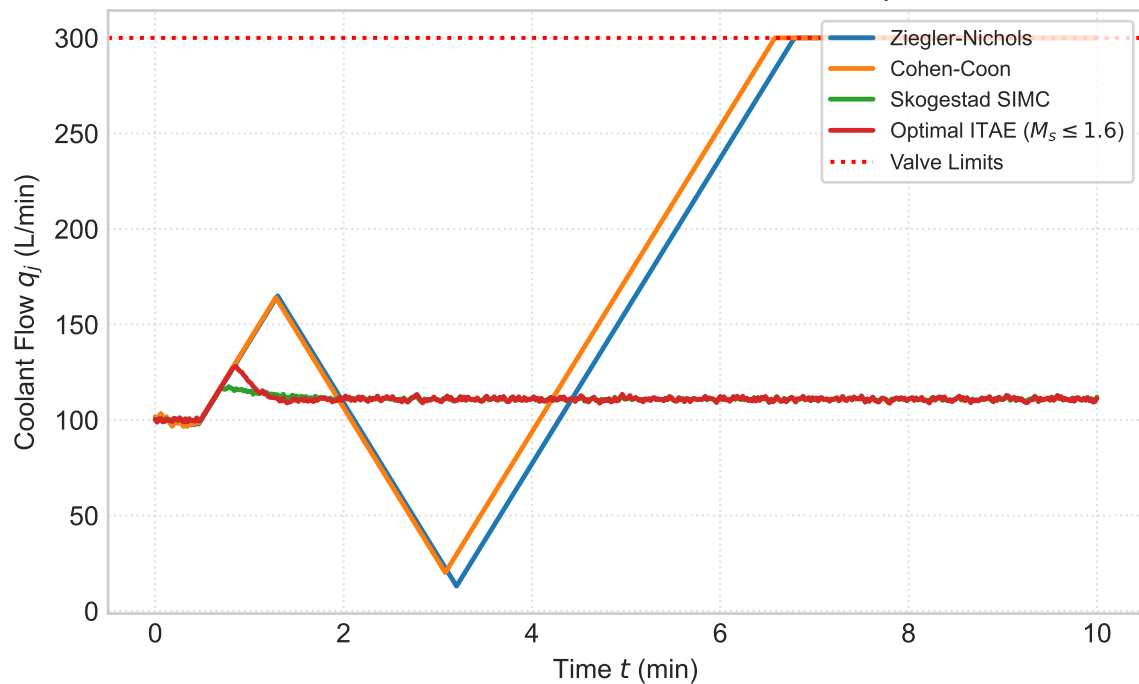
(c) Clean Jacket (100%UA): Coolant q_j
