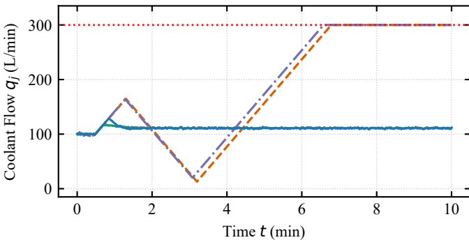
(c) Clean Jacket (100%UA): Coolant q_j
