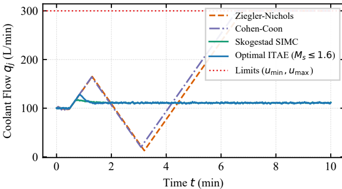
(c) Clean Jacket (100%UA): Coolant q_j
