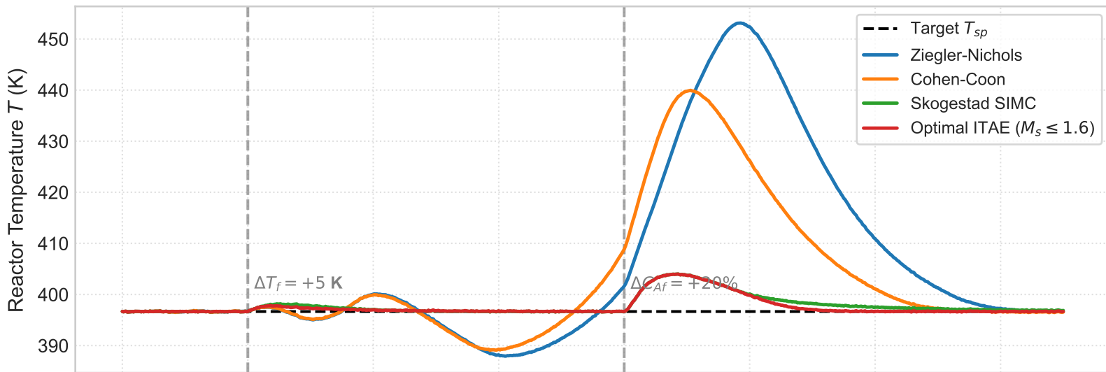
Load Disturbance Rejection: +5 K Feed Temp Surge & +20% Feed Conc Surge
