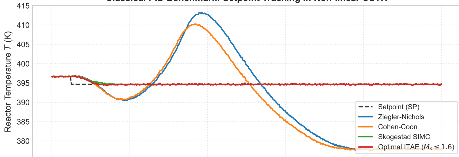
Classical PID Benchmark: Setpoint Tracking in Non-linear CSTR
